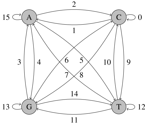
Fig. 1. The weighted De Bruijn graph G_{4,1}(x) corresponding to vector x = (15, 2, 4, 5, 1, 0, 8, 9, 3, 6, 13, 14, 7, 10, 11, 12) , which was introduced in Example 1.
