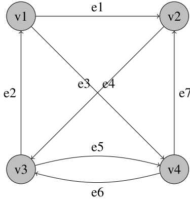
Fig. 3. An example graph with labeled edges.
